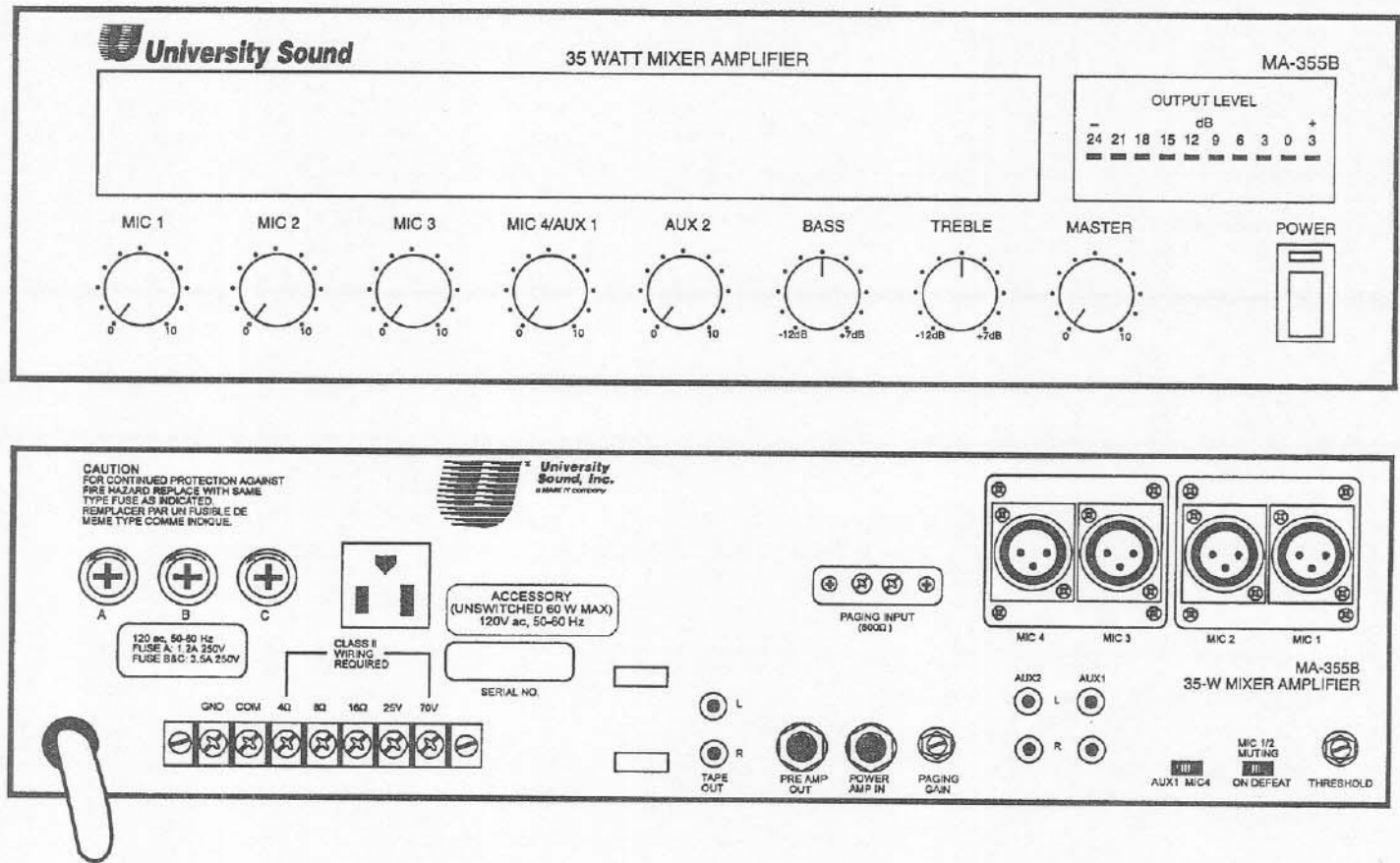
Figure 1—MA-355B Front and Rear Panels
